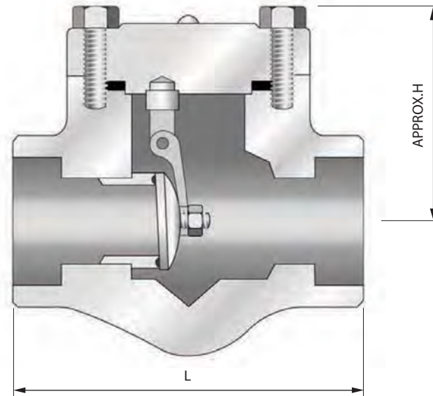
SWING CHECK
