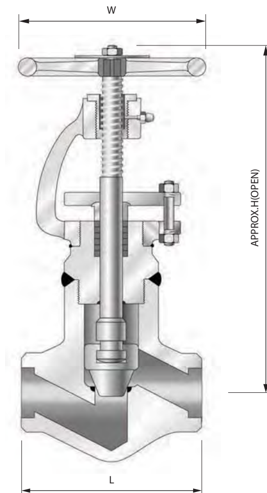
Seal Welded Bonnet
