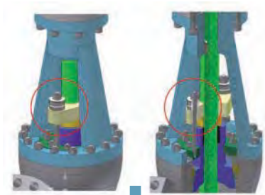
Live-loading
