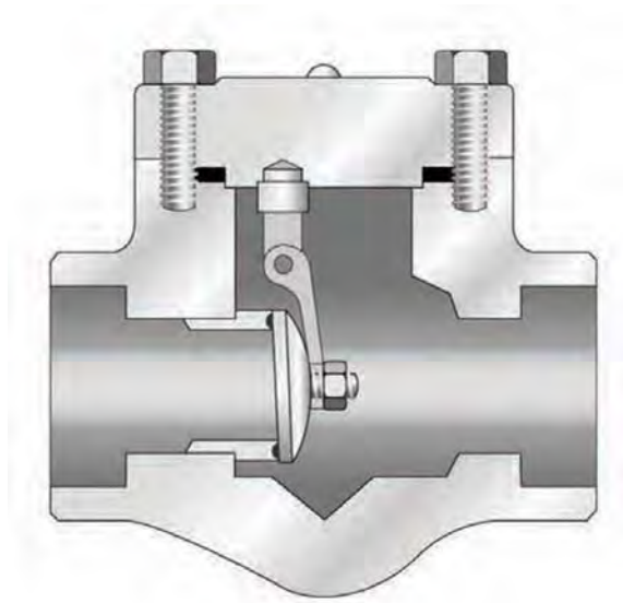
SWING CHECK
