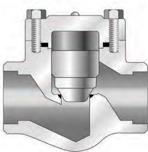
LIFT CHECK
