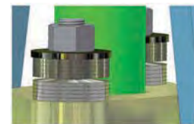
Live-loading Detail
