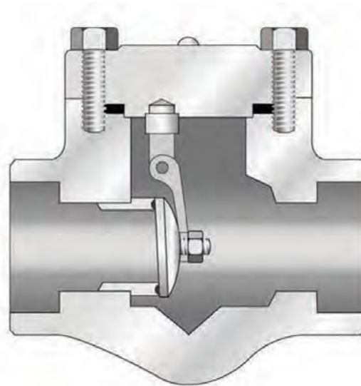
SWING CHECK
