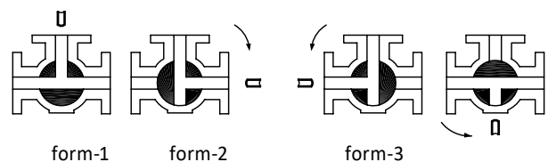
3-way T-Port
