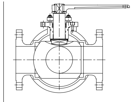
3-way T-Port
