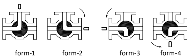
3-way L-Port
