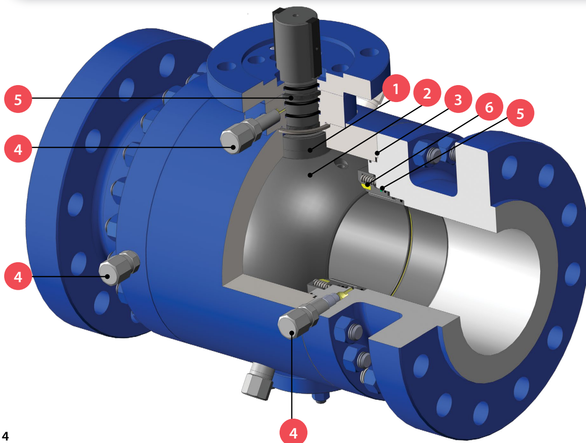
OPTIONAL Double Piston Effect Seats
