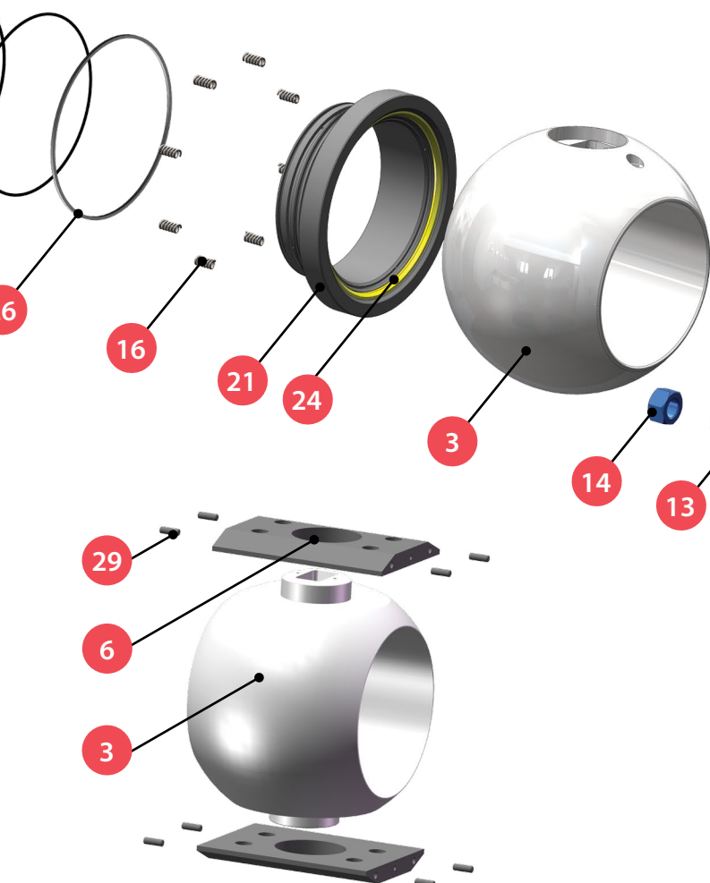
INTERNAL TRUNNION DESIGN Sizes 6"-12" for Class 900 and 1500 Size 14" and larger for all classes
