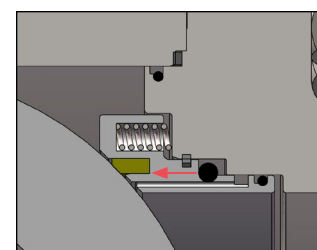
OPTIONAL Double Piston Effect Seats
