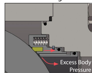
STANDARD Self-Relieving Seats
